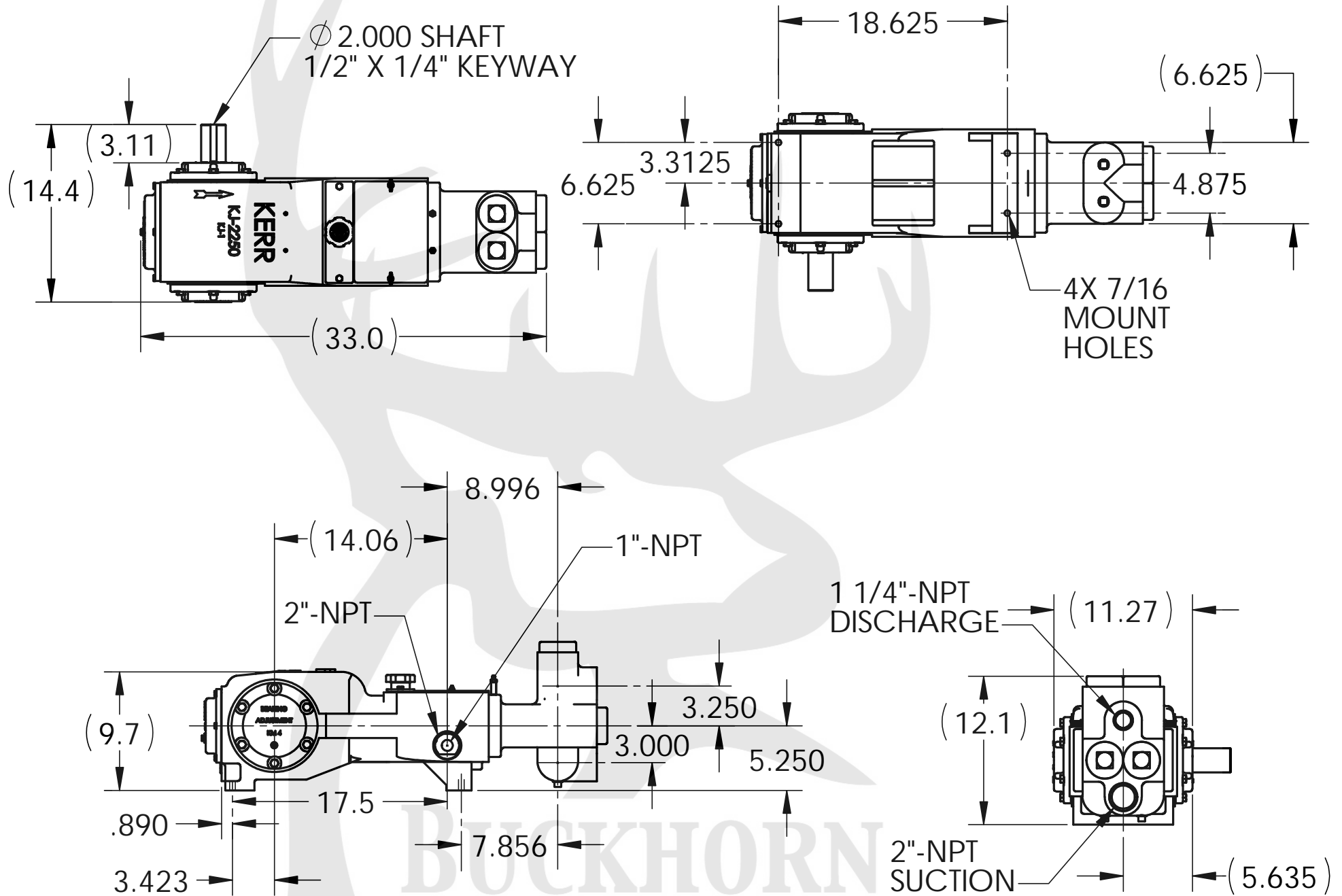
GENERAL DIMENSIONS FOR KJ-2250
