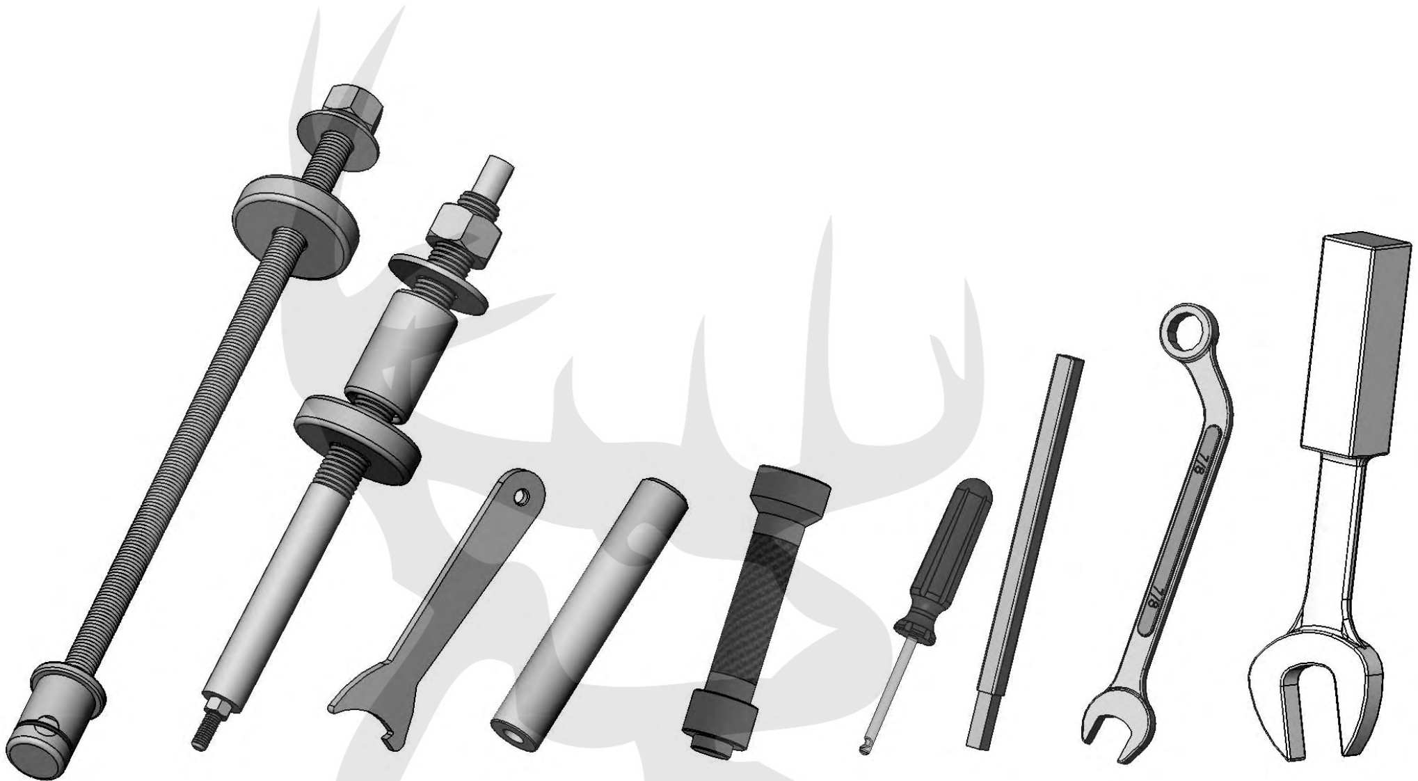
KM-76M WING- GUIDED SEAT TRI-PIN TYPE PULLER ASS'Y
