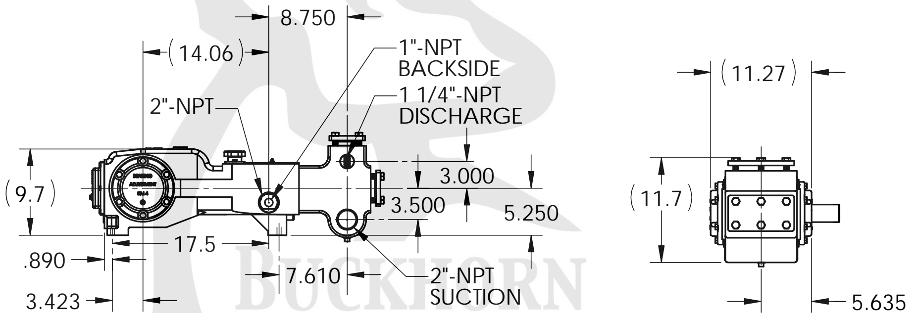
GENERAL DIMENSIONS FOR KJ-2250BC
